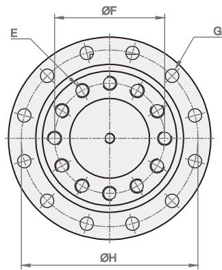
RA30 Rod and Mounting Flange
