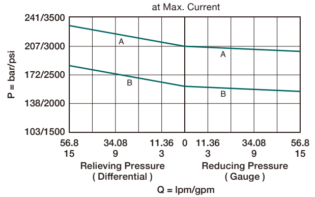
Typical Relieving/Reducing Pressure vs. Flow
