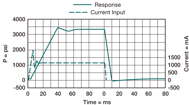
Typical Step Response 207 bar / 3000 psi, 12V Coil, 110 Hz PWM
