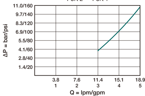
Pressure Drop vs. Flow Port 2 → Port 1
